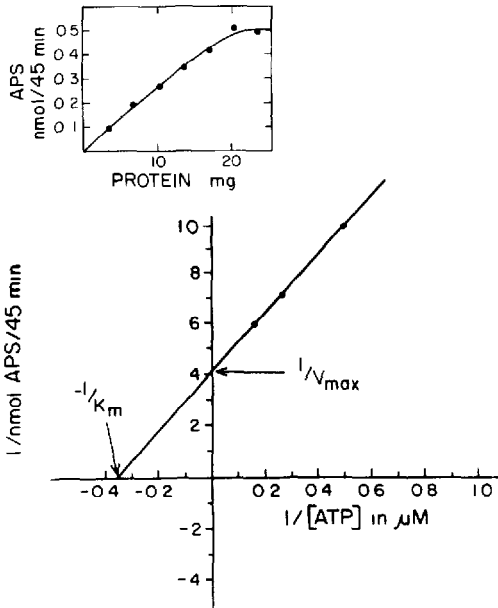
Fig. 6. Kinetic analysis of APS formation by the ATP-sulphyrase. Initial rates of APS formation were determined over a range of ATP concentrations and the results plotted in double reciprocal form. From these data, kinetic constants were determined. The inset shows the rate of APS formation as a function of a protein concentration in the extract.
